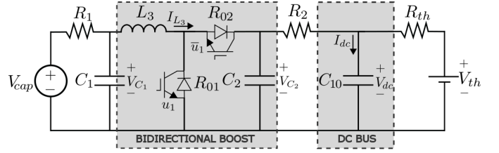
Fig. 2. The simplified electrical model of the DC Microgrid.
