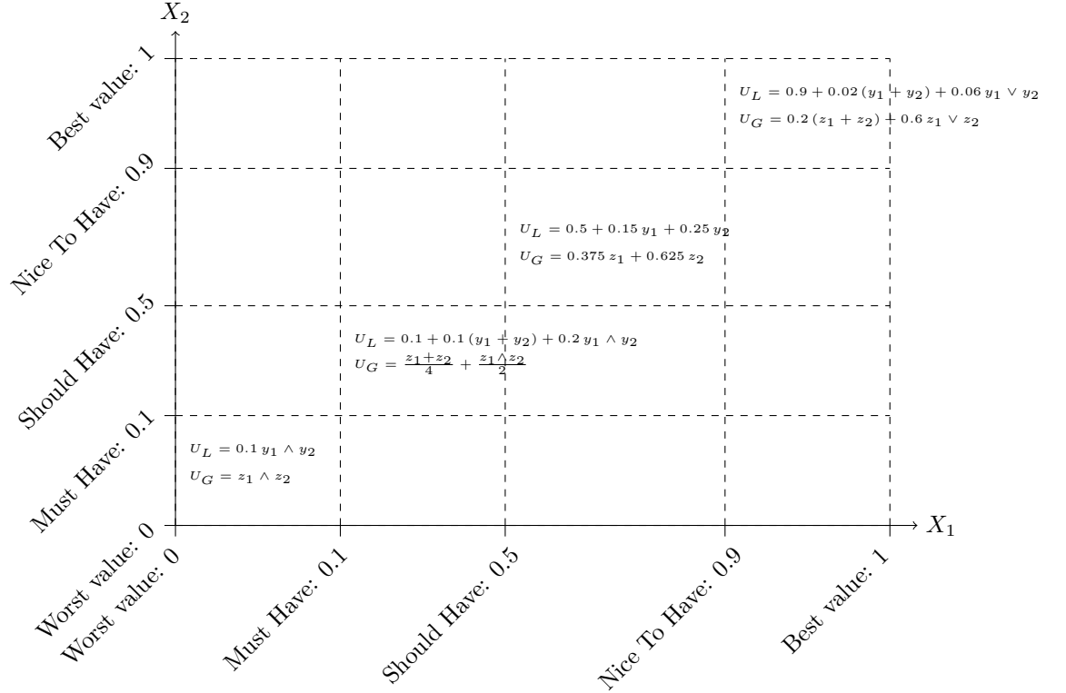
Figure 7: Expression of the overall utility in Example 2. Formula U_v^\wedge(x) = C_{\nu_h}(u_1(x_1) - h, \dots, u_n(x_n) - h) + w(a^h) is written in two different ways. In the first one, we use new variables y_i := u_i(x_i) - h . Then U_v^\wedge(x) is equal to U_L(y) := C_{\nu_h}(y) + w(a^h) (where L refers to the fact that variables y are Local to domain V_q ). The second expression is based on (34). With the new variables z_i = w_i(x_i) , (34) is equal to U_G(z) := C_{\nu_h}\left(\frac{z_1 - w(a^h)}{w(a^{h+1}) - w(a^h)}, \dots, \frac{z_n - w(a^h)}{w(a^{h+1}) - w(a^h)}\right) + w(a^h) (where G stands for Global). The figure presents the two expressions U_L(y) and U_G(z) for the four capacities. They are presented at the four diagonal blocs.
