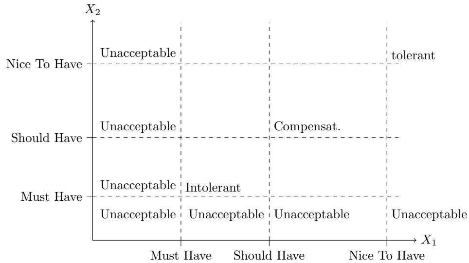
Figure 2: Decision strategies in Example 2.
