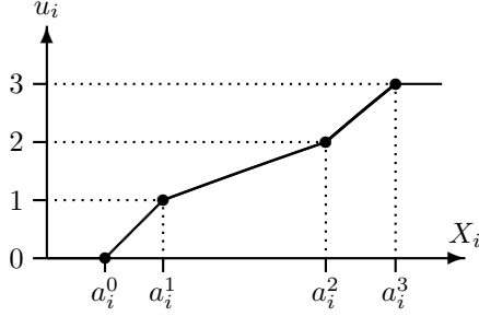
Figure 3: Piecewise affine utility function u_i with p_i = 3 .
