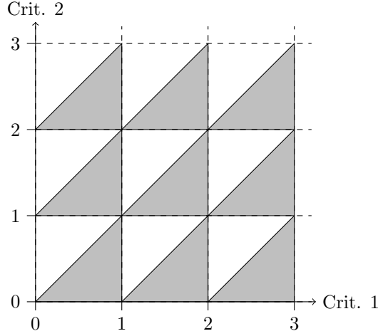
Figure 6: Example with k = 3 . The shaded triangles represent the areas where \phi_1(x) \geq \phi_2(x) .
