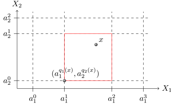
Figure 4: Point x belongs to the square [a_1^1, a_1^2] \times [a_2^0, a_2^1] . Hence q_1(x) = 1 and q_2(x) = 0 .
