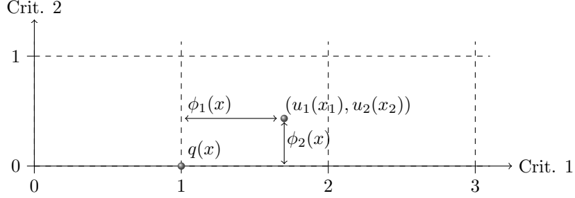
Figure 5: Illustration of q(x) , \phi_1(x) and \phi_2(x) .
