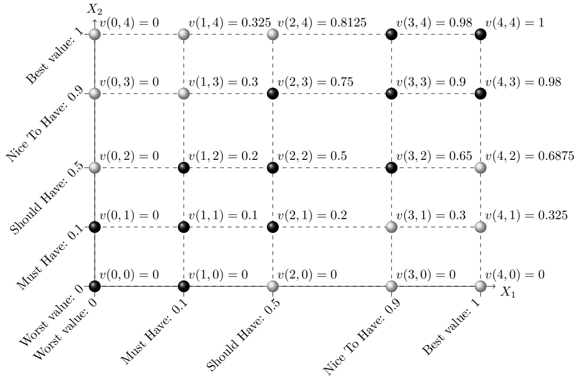
Figure 8: Value of the p -ary capacity in Example 2. The black balls correspond to the values of v that are directly given by \nu_0, \nu_1, \nu_2, \nu_3 . The other values of v (gray balls) are obtained by (35).
