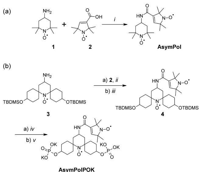
Scheme 1. (a) Synthesis of AsymPol ( 337 \text{ g mol}^{-1} ) a ; (b) Synthesis of AsymPolPOK ( 765 \text{ g mol}^{-1} ) b
