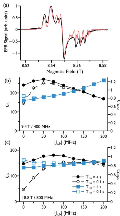
Figure 3. (a) High-field EPR spectrum ( \sim 8.5 T/240 GHz) of 10 mM AsymPolPOK and 20 mM ^{13}\text{C} Urea in d_8 -glycerol/ \text{D}_2\text{O} / \text{H}_2\text{O} (6:3:1; v:v) at 110 K (black) and best fit with a single biradical conformation (red). MAS-DNP simulations of \epsilon_B (black circles) and \epsilon_{\text{DNP}} (blue squares) as a function of the exchange interaction intensity at (b) 9.4 T/400 MHz (c) 18.8 T/800 MHz. The filled symbols were obtained assuming a nuclear relaxation time T_{1,n} = 4 s and the open symbols T_{1,n} = 0.1 s. Lines are added as a guide. Further details of the simulations are provided in the Supporting Information.
