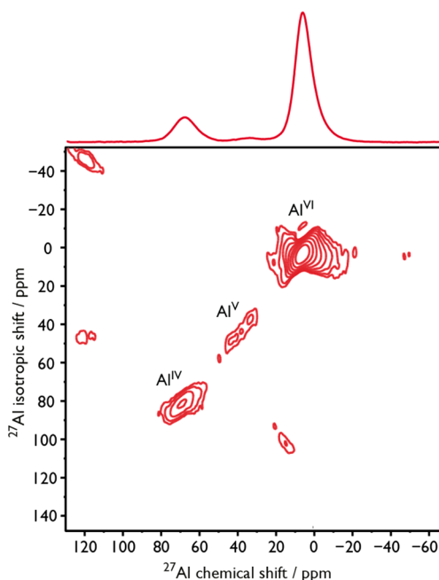
Figure 4. DNP-enhanced \{^1\text{H}\}\text{-}^{27}\text{Al} CP MQMAS NMR spectrum of \gamma -alumina, recorded at 18.8 T, a sample temperature of \sim 125 K, and with a MAS frequency of 24 kHz. Above, a \{^1\text{H}\}\text{-}^{27}\text{Al} CP NMR spectrum of \gamma -alumina recorded under the same conditions as a comparison. The \gamma -alumina was impregnated with a 5 mM AsymPolPOK , 2 M ^{13}\text{C} -urea, d_8 -glycerol/ \text{D}_2\text{O}/\text{H}_2\text{O} (6:3:1; v:v) solution. \varepsilon_{\text{on/off}} = 38 (see Figure S17).
