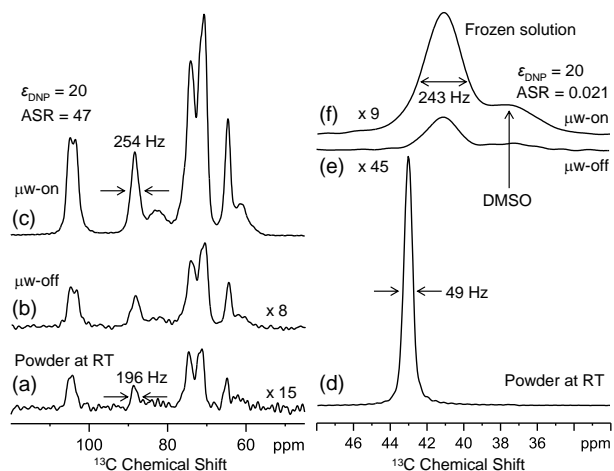
Figure 1. ^{13}\text{C} -CPMAS spectra of NA microcrystalline cellulose (a-c) and 2\text{-}^{13}\text{C} glycine (d-f) recorded on a dried powder for conventional NMR experiments at RT (a, d), a MF sample (b, c) or a frozen solution (e, f) for DNP experiments at 105 K with \mu\text{W-off} (b, e) and \mu\text{W-on} (c, f). The MAS frequency was 8 kHz for all experiments. A DNP enhancement factor, \epsilon_{\text{DNP}} , of 20 was observed with a zirconium rotor although it is 30 % less efficient compared to a sapphire rotor according to DNP experiments on ^{13}\text{C} urea (data not shown).
