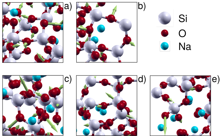
FIG. 5. Visualization of the vibrational modes at (a) 416\text{ cm}^{-1} , (b) 481\text{ cm}^{-1} , (c) 602\text{ cm}^{-1} , (d) 694\text{ cm}^{-1} and (e) 976\text{ cm}^{-1} for the NS4 glasses. White atoms are Si, red are O, and blue are Na. For the color version, the reader is referred to the web version of the paper.
