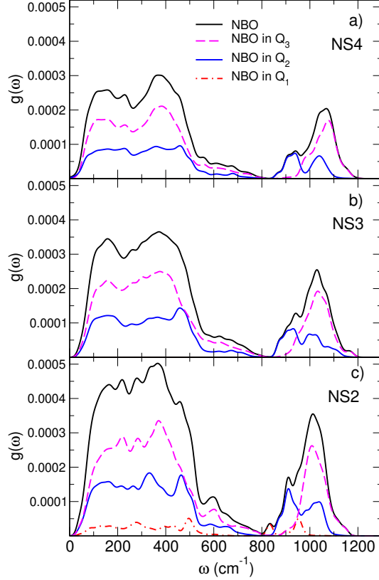
FIG. 9. Contributions to the NBO partial VDOS of NBO's on Q_2 and Q_3 -species for (a) NS4, (b) NS3, and (c) NS2.
