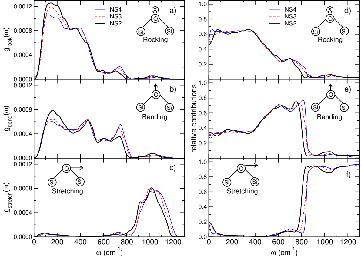
FIG. 7. Frequency and composition dependencies of the (a) rocking, (b) bending, and (c) stretching components of BO modes in the three NSX glasses ( X=4,3,2 ). (d)–(f) show the relative contributions of the rocking, bending and stretching motions, respectively, with respect to the total VDOS.
