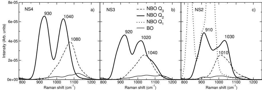
FIG. 14. Per-atom contribution to the Raman spectra of NBO's on different Q_n -species for (a) NS4, (b) NS3, and (c) NS2. The per-atom contribution of BO's is also given for comparison. The maxima of the contributions for Q_2 and Q_3 species are noted on the plots.
