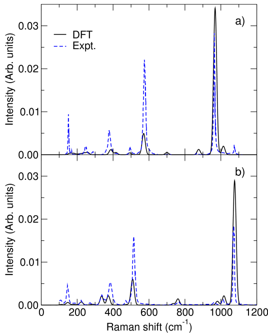
FIG. 1. Polarized Raman spectra for a) \text{Na}_2\text{SiO}_3 and b) \alpha\text{-Na}_2\text{Si}_2\text{O}_5 . Experimental spectra are from Refs. 51,52 .
