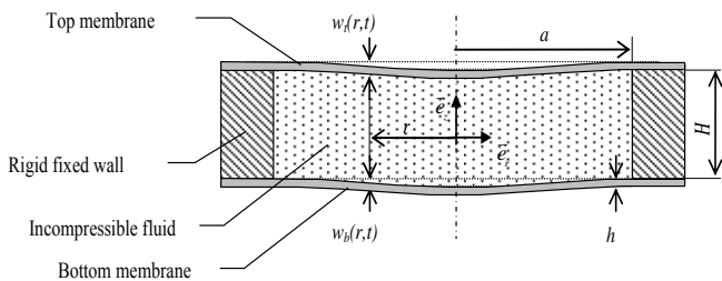
Figure 1: Hybrid fluid diaphragm schematic
