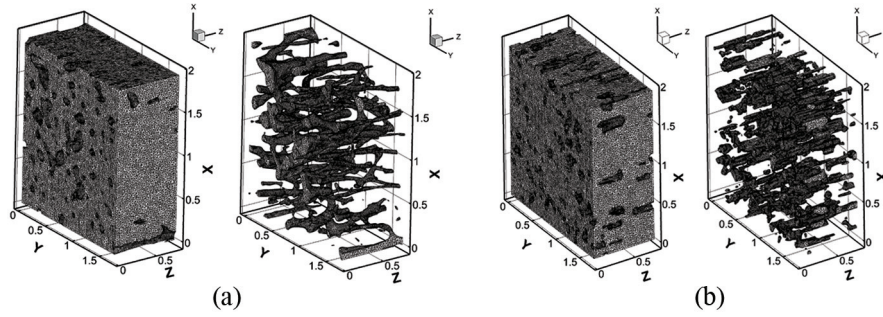
Figure 3. Finite element mesh for cortical bone microstructures (left: bone phase, right: void phase): (a) real specimen; (b) statistically reconstructed specimen from cut section 2. The approximate size of samples (real and reconstructed ones) is 1930 \times 1750 \times 600 \mu\text{m}^3 .
