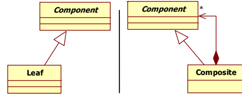
Figure 9. The Composite pattern without Composite and without Leaf
