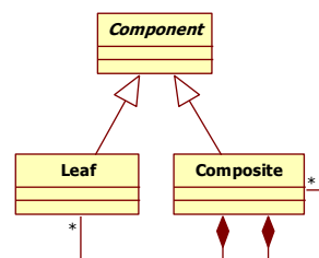
Figure 1. A spoiled pattern (development of the composition on Composite )
