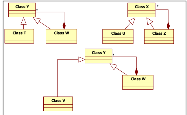
Figure 6. Sub-fragments of Fig.4 isomorphic with the pattern of Fig. 3
