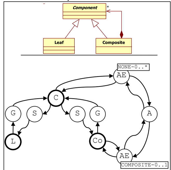
Figure 3. A UML model and its directed graph representation
