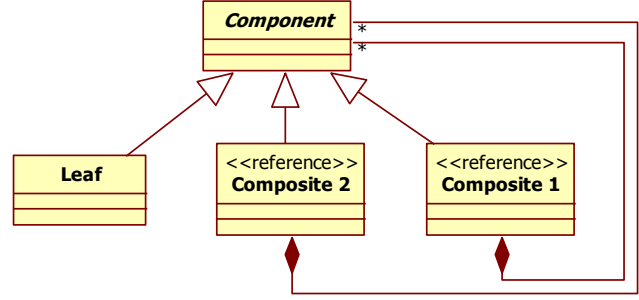
Figure 8. A particular case of a complete fragment
