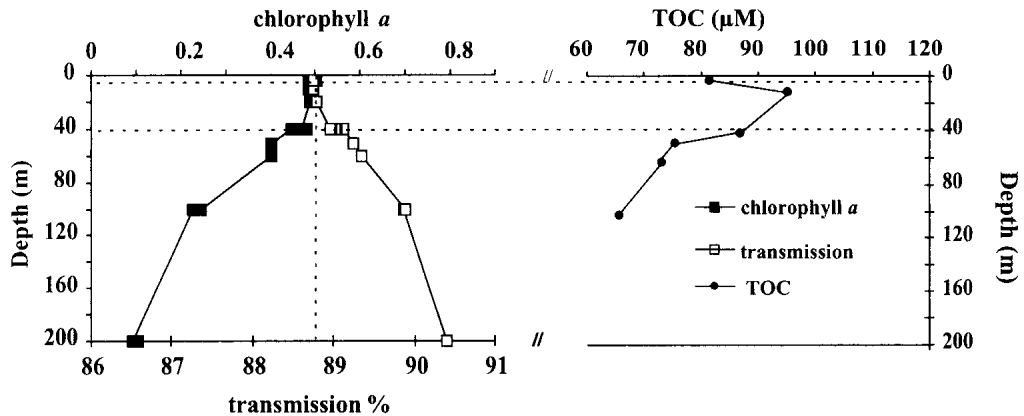
Fig. 2. Chlorophyll a and transmission and TOC profiles in Mediterranean, Frontal, and Atlantic waters of the Almeria-Oran Front. The horizontal dashed lines indicate the sampling depth for colloid determinations.
