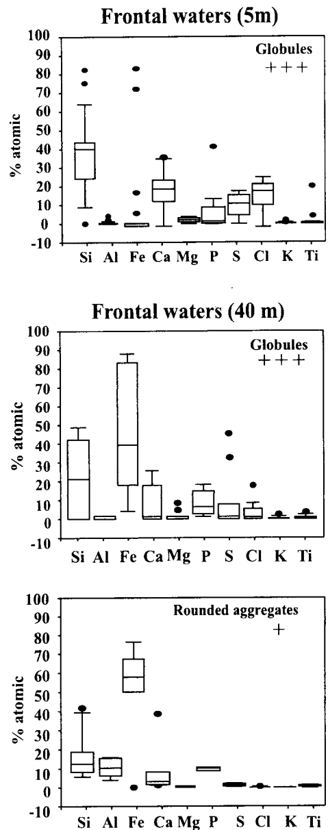
Fig. 7. Box plot representations of the chemical composition of the different colloidal morphotypes encountered in Frontal waters (abundance: +++ high, + low).
