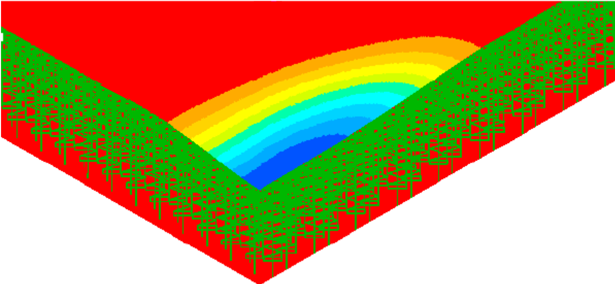
Figure N° 8: Shape of the dent at the critical load.
