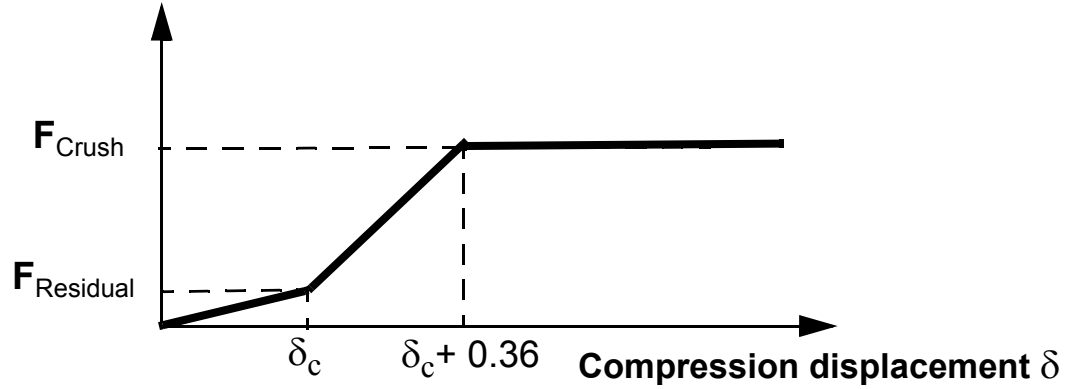
LAW B: Spring force for a damaged honeycomb
