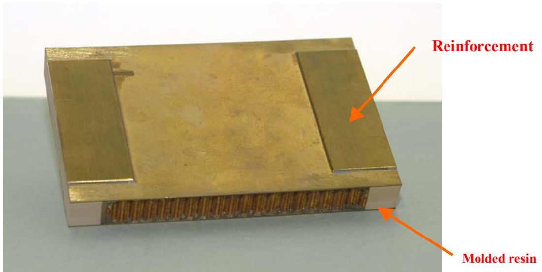
Figure N° 1 : Sandwich with metallic skins used for CAI Tests ([19]).
