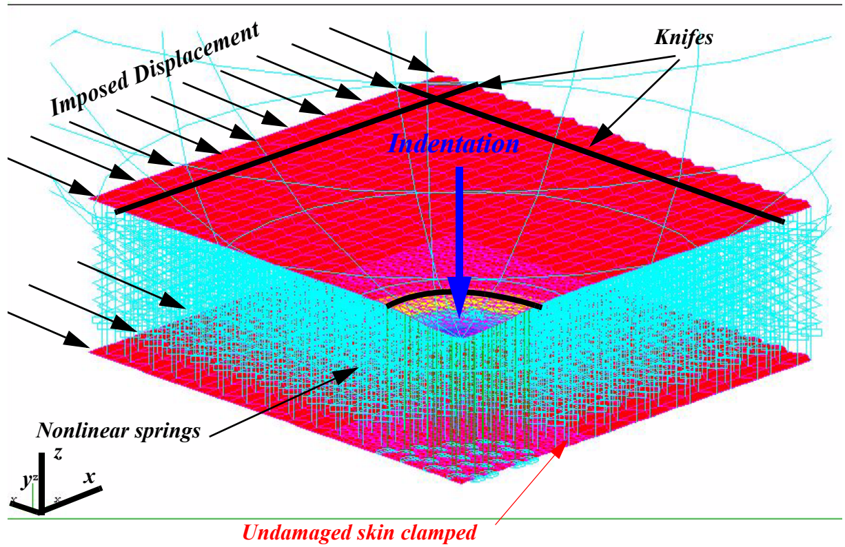
Figure N° 2: Finite element model for compression-after-impact of sandwich with metallic skins.
