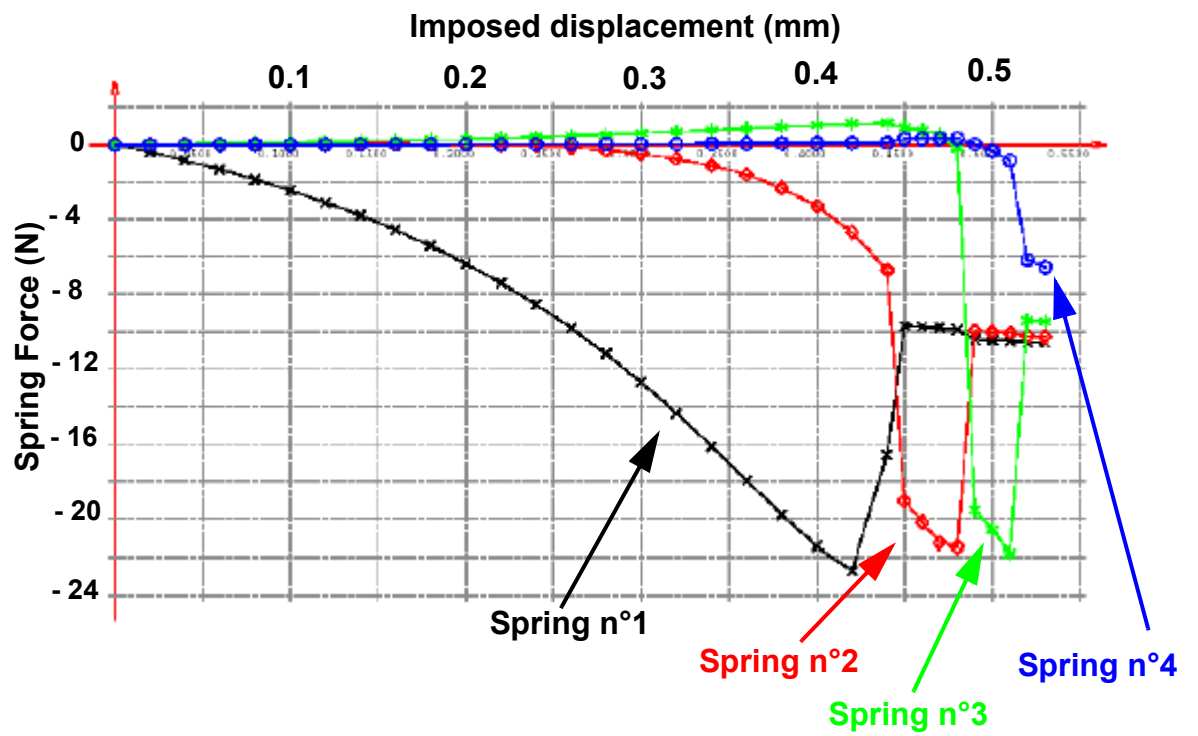
Figure N° 7: Typical response given by the model (case n°4).
