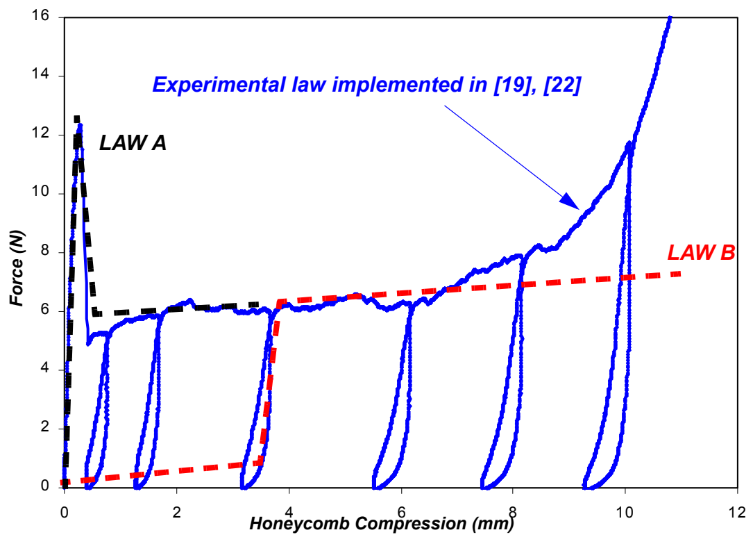
Figure N° 3: Compression behaviour of Nomex honeycomb with cycling.
