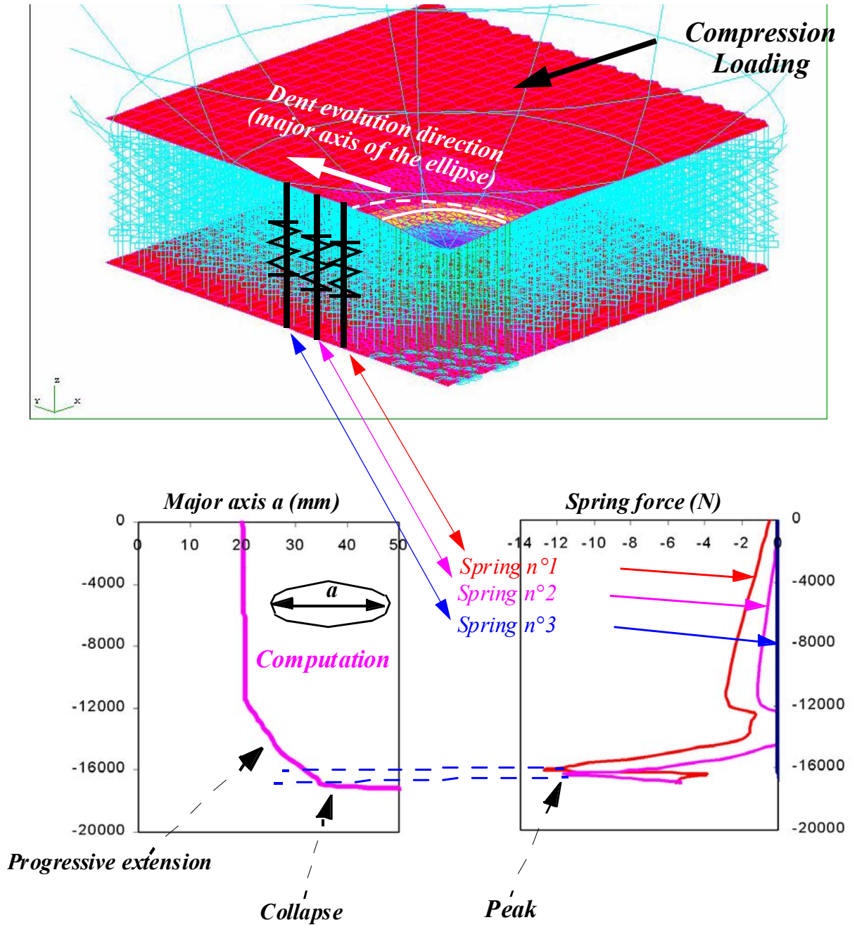
Figure N° 4: Core crush criterion.
