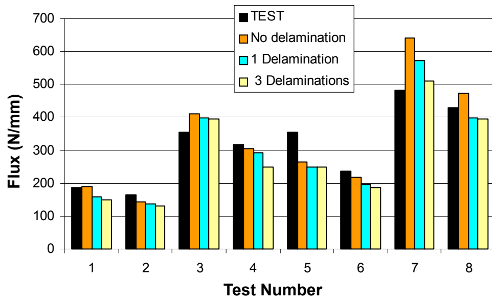
Figure N° 10: Bending stiffness in the damaged skin influence.
