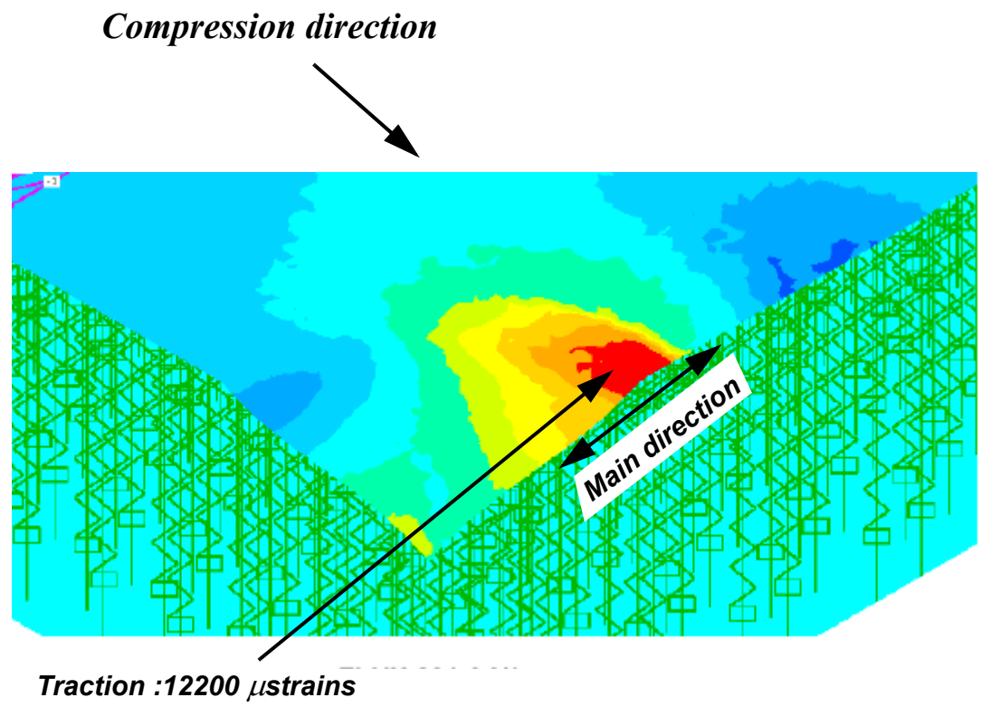
Figure N° 9: Main strain field, lower skin, critical load 291.5 N/mm.
