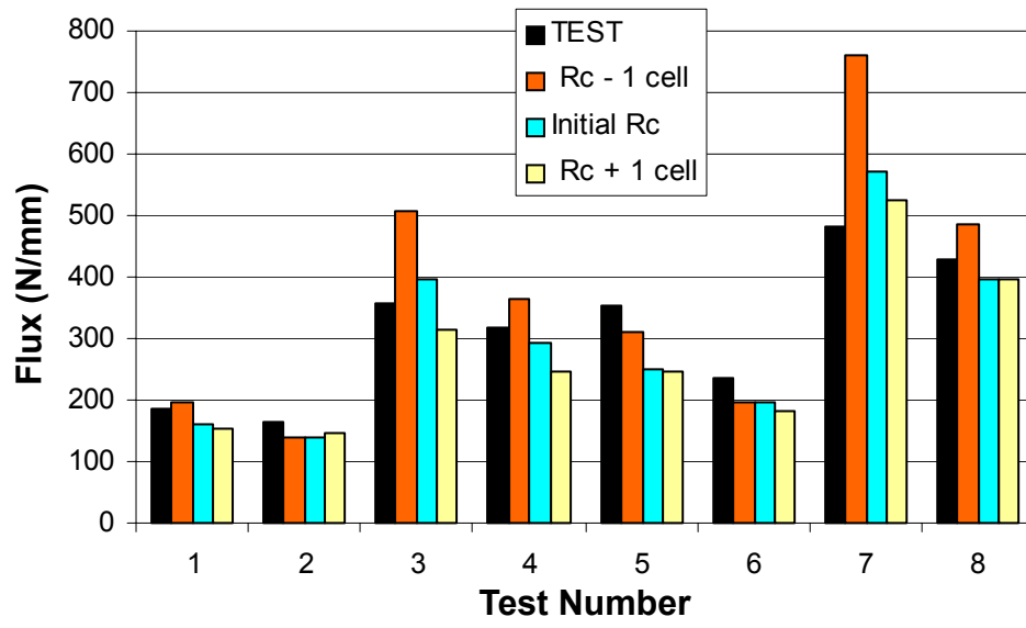
Figure N° 11: Core crush radius influence.
