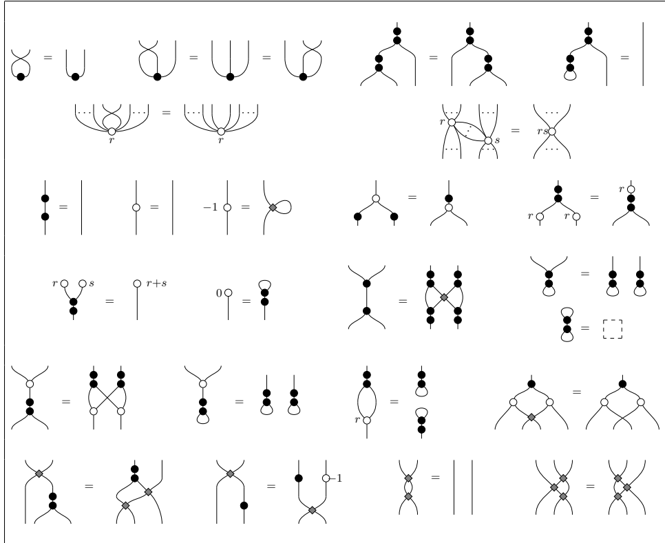
Fig. 1. Set of rules for the ZW-Calculus. r, s \in \mathbb{C} .
