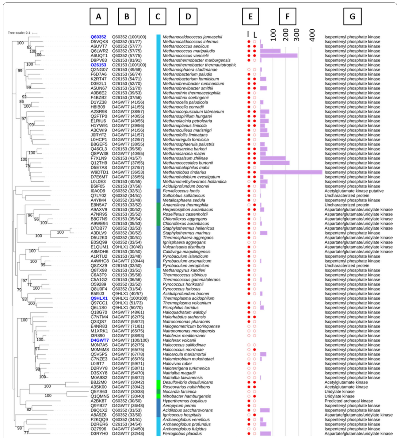
Fig. 1 Phylogenetic tree of 82 cloned IPK candidates from biodiversity compared with IPKs from literature. Bootstrap values expressed as a percentage of 1000 replications are shown next to each node if value > 75%. a UniProt identifiers of each candidates. The 4 IPKs from literature used as the reference set in the sequence driven approach are noted in blue. b Best hit from IPK reference set and its percentage of identity and homology with the candidate. c Phylogenetic lineage of IPKs: Archaea are in blue (light blue: Euryarchaeota ; dark blue: Crenarchaeota ) and bacteria are in green (light green: Proteobacteria ; dark green: Terrabacteria group). d Selected microorganisms. e Protein expression status according SDS gel analysis of cell free extract by eye. "I" full red dot means that the protein was visibly induced by IPTG treatment and "L" means that the protein is visibly present in the cell free extract. f Quantification by LC/MS analysis of IPP/DMAPP production ( \mu\text{M/L} ) in 96-microwell screening. g Protein name according to UniProt annotation
