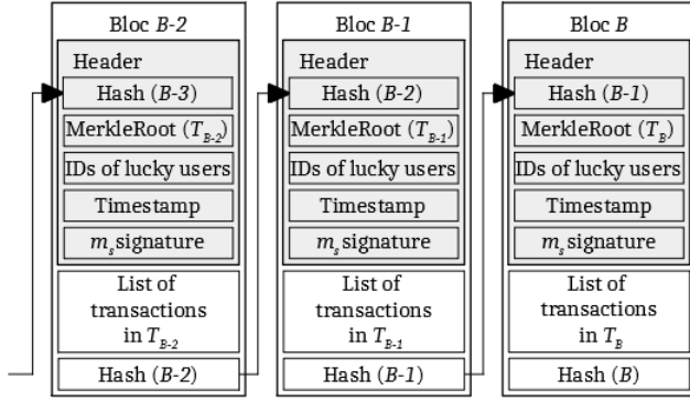
Fig. 9. Structure of the blockchain.
