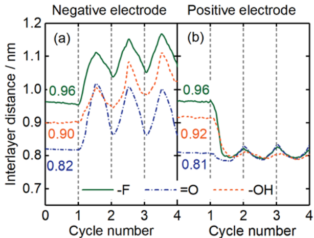
Figure 3. Evolution of the average interlayer distances between the \text{Ti}_3\text{C}_2\text{T}_x layers of both negative and positive electrode during the neutral cycle (0 - 1 cycle) and galvanostatic charge/discharge cycles (1 - 4 cycles). A 9 galvanostatic charge/discharge cycles' simulation result is shown in Figure S3 in supporting information.
