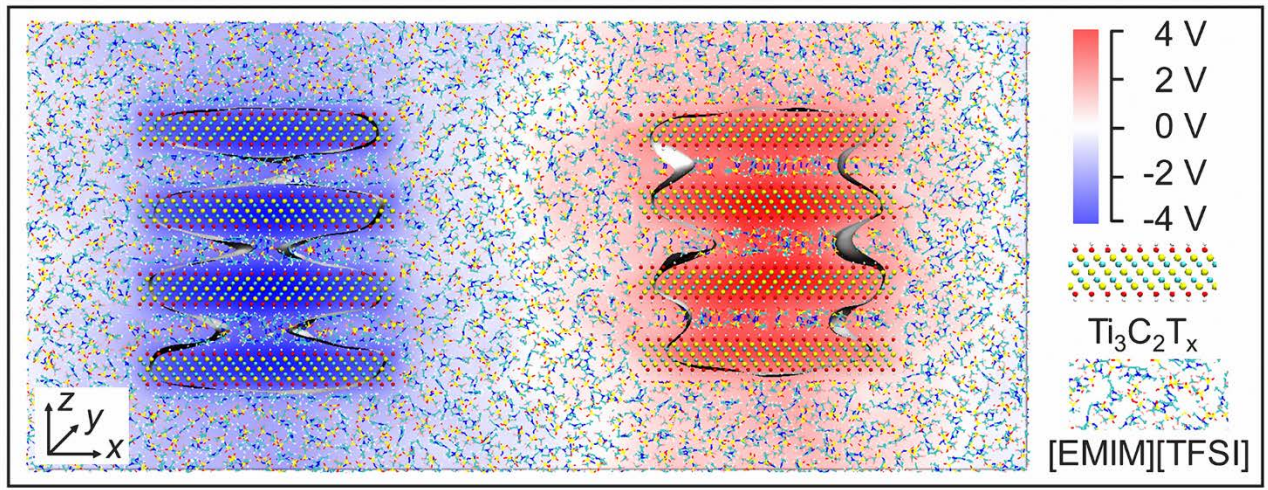
Figure 1. Snapshot of the simulation system obtained using the VMD software [20] . The system consists in a negative electrode (four layers of Ti 3 C 2 T x on the left), a positive electrode (four layers of Ti 3 C 2 T x on the right), and a pure ionic liquid ([EMIM][TFSI]) surrounding the electrodes. The color spectrum, with blue as the lowest electrostatic potential value and red as the highest, is employed to convey the varying intensities of the electrostatic potential values. The silvery wavy surfaces surrounding the Ti 3 C 2 T x layers represent the electrostatic isopotential surfaces of -2 V (negative electrode) and +2 V (positive electrode).
