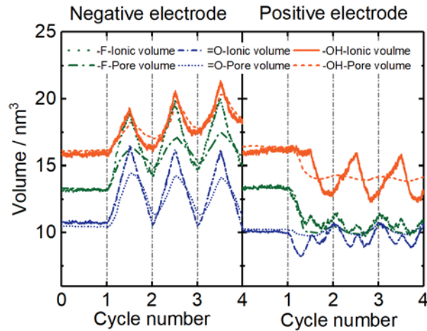
Figure 6. Change of electrode pore volume (dashed line) and in-pore ionic volume (solid line) in both negative and positive electrode pores during the OCV period (0 -1 cycle) and galvanostatic charge/discharge cycles (1 - 4 cycles).
