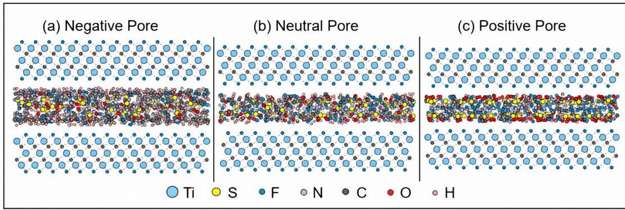
Figure 7. Snapshots of the ionic arrangements inside one of the Ti 3 C 2 F 2 electrode pores at different charged state: (a) negatively charged, (b) neutral, (c) positively charged, respectively.
