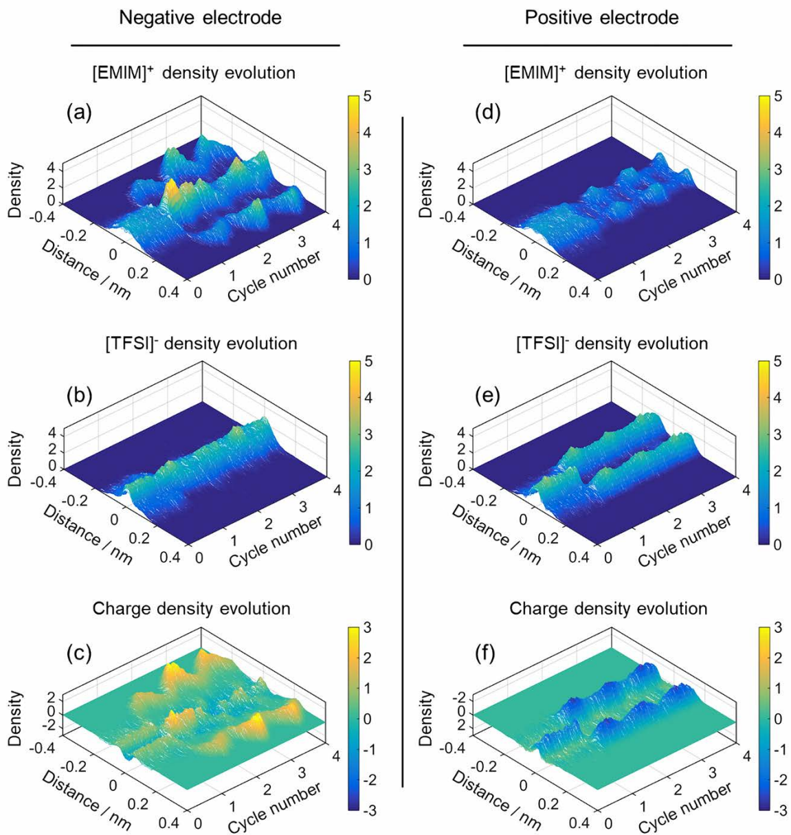
Figure 8. Evolution of [EMIM] + , [TFSI] - density profiles and charge density profiles inside the negative electrode pore ((a), (b), (c)) and positive electrode pore ((d), (e), (f)) of Ti 3 C 2 F 2 electrode during neutral e (0 - 1 cycle) and charge/discharge process e (1 - 4 cycle), as an example.
