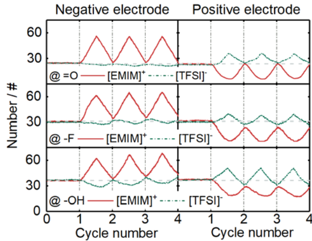
Figure 4. Evolution of the [\text{EMIM}]^+ and [\text{TFSI}]^- ion populations inside the pores for both the negative and positive electrodes during the neutral cycle (0 - 1 cycle) and the galvanostatic charge/discharge cycles (1 - 4 cycles).
