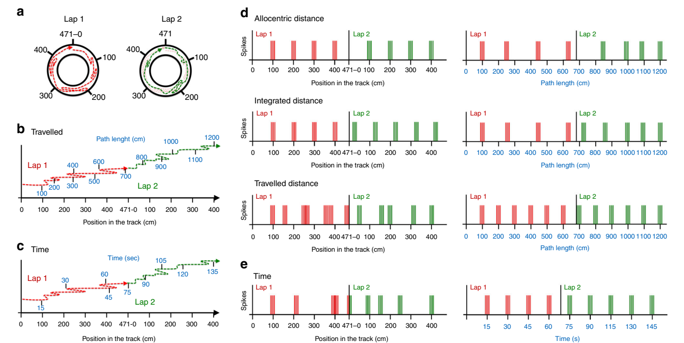
Fig. 1 Predictions of grid cell firing based on allocentric distance, path integrated distance or travelled distance models. a Hypothetical trajectory of a rat in the circular track; red and green represent the first and the second lap, respectively. The total length of the track (471 cm) as well as cumulative 100 cm distances are indicated. b, c Hypothetical trajectory of a rat as a function of the position in the track. The blue values indicate the cumulative travelled distance ( b ) or the cumulative time elapsed ( c ), for each lap. The trajectories corresponding to the first and second laps are indicated in red and green, respectively. d Hypothetical position of grid cell firing fields relative to the track (left diagrams) or to the travelled path (right diagrams). Top row: according to the allocentric distance model, the firing fields keep the same position in the track across different laps (left), whereas their position relative to the cumulative travelled distance is highly variable from one lap to the other (right). Middle row: according to the path integrated distance model, the distance between the firing fields across laps is constant relative to the track (left), whereas their position relative to the animal path is highly irregular (right). Bottom row: according to the travelled distance model, firing fields are irregularly distributed around the track (left) but show a constant spacing across laps relative to the path travelled (right). e According to the time model, grid cells are expected to fire regularly based on a constant time step (right), and irregularly relative to the track positions (left)
