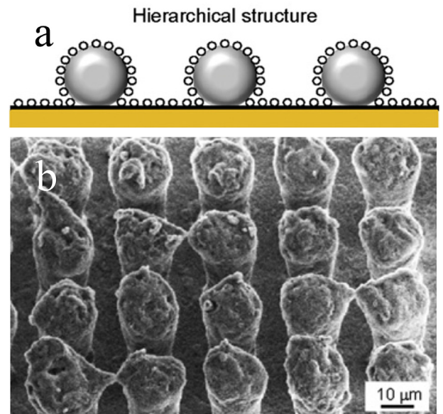
Fig. 19. Bimodal surface structures consisting of (a) two powder particle sizes and (b) surface structure created with lithography and spraying of nano-sized silica. Figures reproduced from Ref. [73] with permission from Elsevier.
