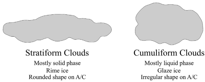
Fig. 2. Ice characteristics for stratiform and cumuliform clouds.
