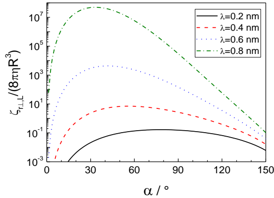
Figure 6 Rotational line friction \zeta_{r\perp,L} divided by the bulk Stokes rotational friction as a function of the particle contact angle for different values of the contact line displacement \lambda .
