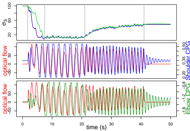
Fig. 2. Above, evolution of \sigma_s : in red and blue for the shoulder CPG; in green and purple for the elbow CPG. Note that the extensor and flexor curves are merged for both CPGs. Below, in red, the optical flow detected. In blue, the position command sent to the shoulder joint. In green, the position command sent to the elbow joint.
