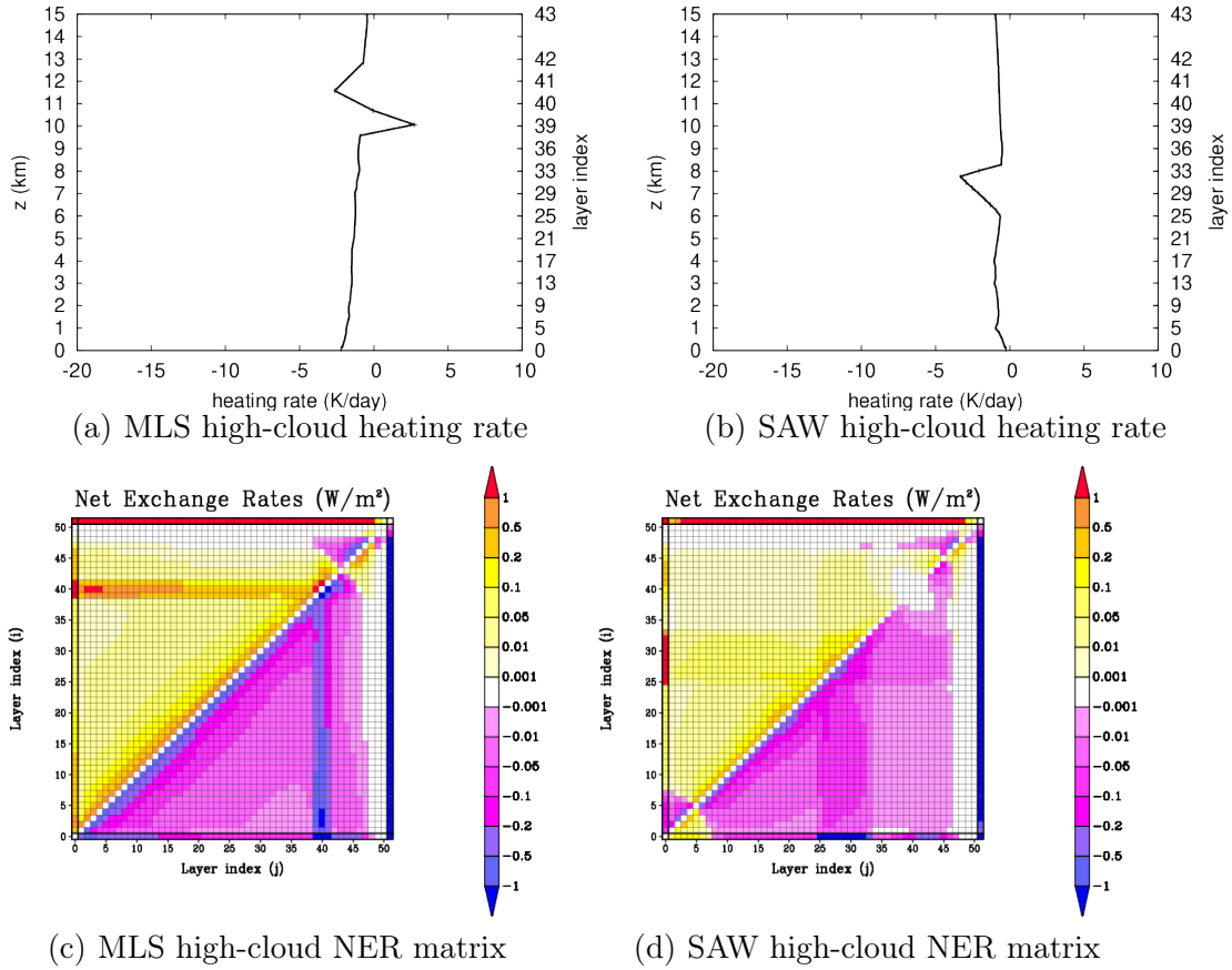
Fig. 8. (a): heating rate ( K/day ) for MLS high-cloud configuration (ice cloud extending from 10.0 to 12.0km (layers 39 – 41) with IWC = 0.0048g.m^{-3} and D_e = 41.5\mu m ) ; (b): same as (a) for SAW atmosphere (water cloud extending from 6.0 to 8.0km (layers 25 – 33) and same IWC and D_e ) ; (c): NER matrix ( W/m^2 ) in the high-cloud configuration for a MLS atmospheric profile ; (d): same as (c) for a SAW atmospheric profile.
