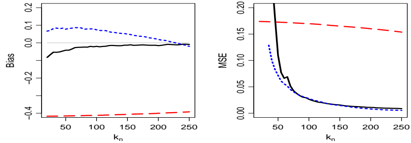
(c) Weibull(2) censored by Weibull(5), where \theta_X = 1/2 and \theta_C = 1/5 .
