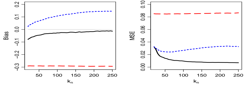
(b) Weibull(2) censored by Weibull(2), where \theta_X = 1/2 = \theta_C .
