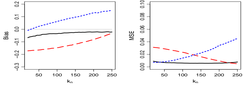
(a) Weibull(2) censored by Weibull(2/3), where \theta_X = 1/2 and \theta_C = 3/2 .
