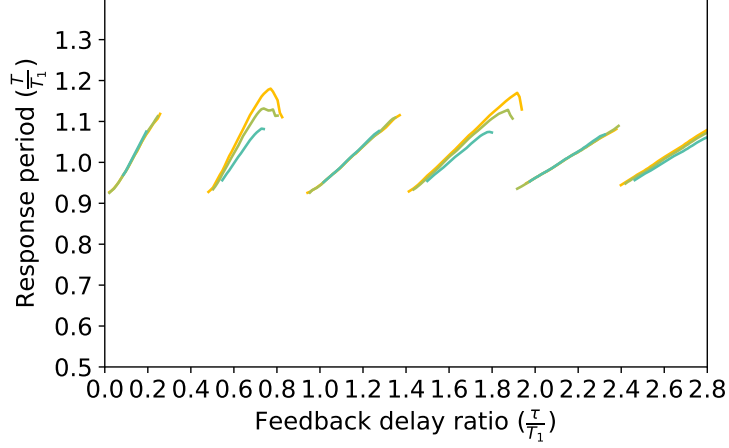
Figure 7: Oscillation period over first natural period as feedback delay ratio \tau/T_1 is varied for different Kelvin-Voigt damping coefficients. \eta = 0.005 s (orange), \eta = 0.010 s (green), \eta = 0.020 s (blue). \chi = 7.5 \text{ N} \cdot \text{m} \cdot \text{rad}^{-1} .
