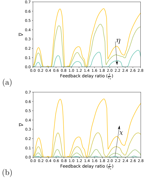
Figure 6: Mean forward velocity \bar{V} as feedback delay ratio \tau/T_1 is varied (a) for different Kelvin-Voigt damping coefficients. \eta = 0.005 s (orange), \eta = 0.010 s (green), \eta = 0.020 s (blue), for \chi = 7.5 \text{ N} \cdot \text{m} \cdot \text{rad}^{-1} . (b) as \chi is varied \chi = 3.25 \text{ N} \cdot \text{m} \cdot \text{rad}^{-1} (blue), \chi = 5.0 \text{ N} \cdot \text{m} \cdot \text{rad}^{-1} (green), \chi = 6.25 \text{ N} \cdot \text{m} \cdot \text{rad}^{-1} (beige), \chi = 7.5 \text{ N} \cdot \text{m} \cdot \text{rad}^{-1} (orange), for \eta = 0.005 s
