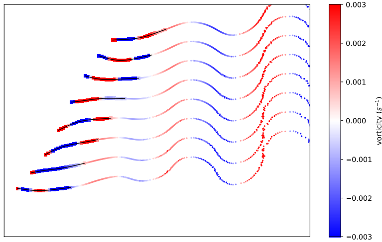
Figure 3: Vorticity distribution of the swimmer and its wake over approximately one period. \eta = 0.005 s, \frac{\tau}{T_1} = 2.17 and \chi = 10 N · m · rad -1 .
