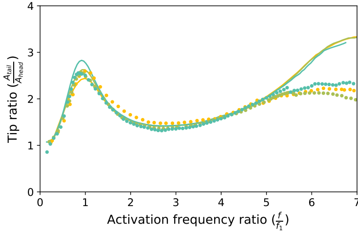
Figure 4: Tail amplitude response A_{\text{tail}} normalized by the imposed head amplitude A_{\text{head}} as a function of the ratio of the heave frequency to the first natural frequency for a heave amplitude of A_{\text{head}} = 0.004 m and Reynolds number of 6000. EI = 0.018 (orange), EI = 0.028 (green), EI = 0.053 (blue). Curves: results of present work. Disks: results of Paraz et al. [29].
