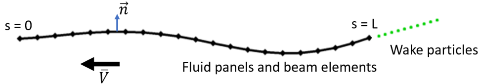
Figure 1: The swimmer is modeled by an Euler-Bernoulli beam which is discretized into beam elements and fluid panels while its wake is represented with point vortices.
