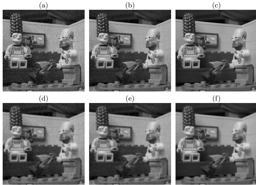
Figure 1: (a) noisy image (standard deviation 30/255 ). (b) denoised with HDMI [1] (patches 7 \times 7 ), PSNR = 31.92 dB. (c) image from the denoised patches of (b) with DC component corrected with oracle value (f) , PSNR = 33.78 dB. (d) DC component of the patches of (a) . (e) DC component of the patches of (b) . (f) DC component of the oracle image (ground truth).
