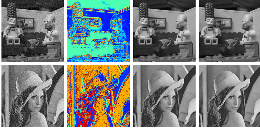
Figure 3: From left to right. Noisy images (standard deviation 30/255). HDMI resulting groups. HDMI denoised (lena 31.09dB, simpson 32.46dB). Denoising with method 4.2.1 (lena 31.19dB, simpson 32.58dB).
