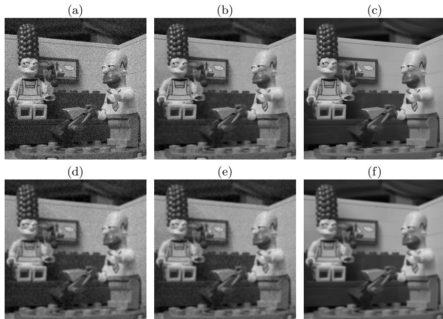
Figure 1: (a) noisy image (standard deviation 30/255 ). (b) denoised with HDMI [1] (patches 7 \times 7 ), PSNR = 31.92 dB. (c) image from the denoised patches of (b) with DC component corrected with oracle value (f) , PSNR = 33.78 dB. (d) DC component of the patches of (a) . (e) DC component of the patches of (b) . (f) DC component of the oracle image (ground truth).
