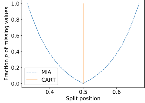
Figure 1: Split position chosen by MIA and CART criterion, depending on of the fraction p of missing values on X_1 .
