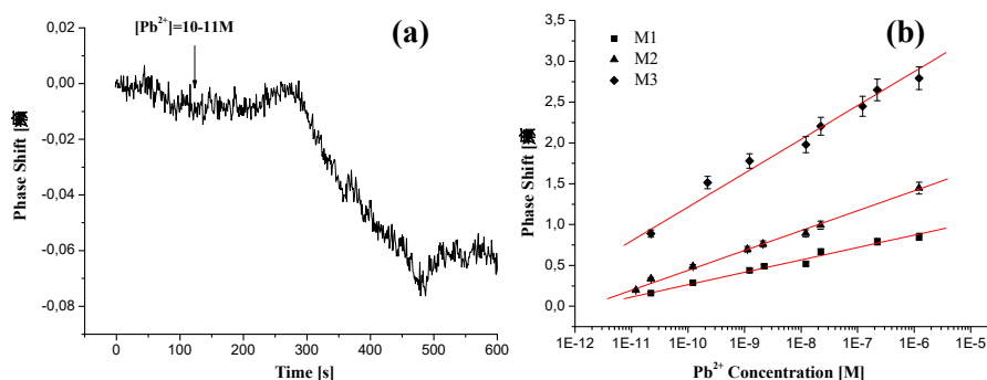
Figure 1. (a) Phase variations versus time after the injection of a solution of 10^{-11} M of Pb^{2+} on the sensing area of a M1/SAW sensor (b) Semi-logarithmic phase-shift variations ( \Delta\Phi ) versus lead ions concentration for the M1, M2 and M3/SAW sensors.
