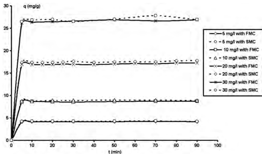
Fig. 2. Effect of the initial concentration of MB on the kinetics of elimination with FMC and SMC at W_a = 1 \text{ g/l} ; \text{pH} = 7 and T = 20^\circ\text{C} .
