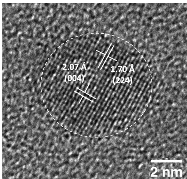
Figure 5. High-resolution transmission electron microscopy view of a representative particle ( x = 0 ) of the produced nanocrystalline Co 0.6 Zn 0.4 Fe 2-x Gd x O 4 solid solution, with the indication of some reticular distances matching well with the Co 0.6 Zn 0.4 Fe 2 O 4 spinel structure (ICDD no. 98-016-6202).
