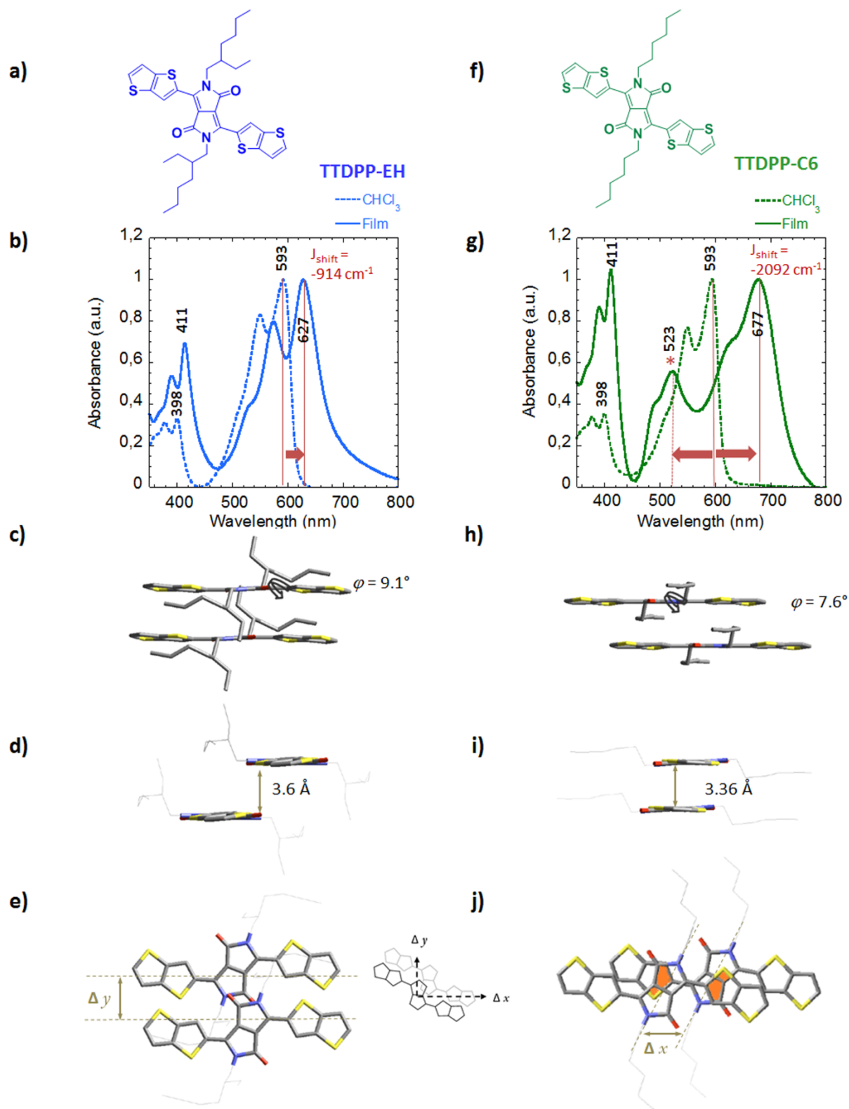
Figure 1: Chemical structures and comparison of the packing behavior in the solid state of TTDPP-EH (a-e) and TTDPP-C6 (f-j). b, g) Changes in the absorption spectra from dilute solution (in chloroform, dashed lines)
