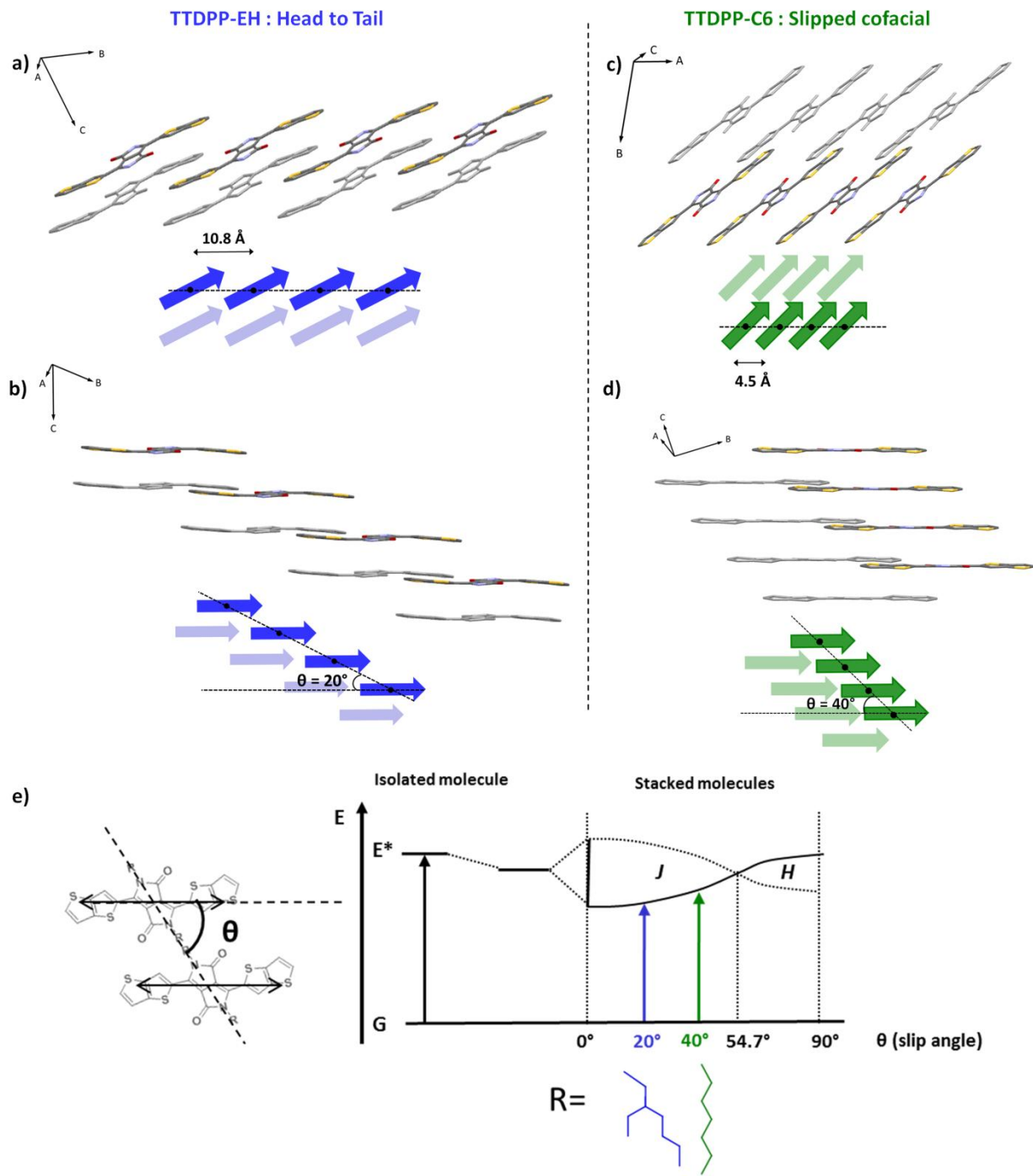
Figure 2: Representation of two stacks of 4 molecules taken from the crystal structures of TTDPP-EH (a, b) and TTDPP-C6 (c, d) and schematic illustrations of phase relations transition dipole moments. (Side chains and H are omitted for clarity; the next layers of molecules are represented in grey in the structure and pale color in the schematics). The center-to-center distances between neighbor molecules are 10.8 Å and 4.5 Å and
