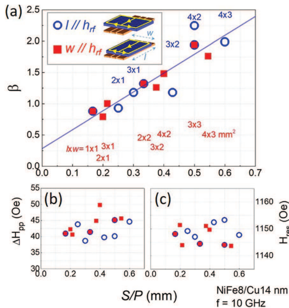
FIG. 3. (a) Dependences of \beta on the ratio S/P for Si/SiO 2 /NiFe(8)/Cu(14)/Al(2)Ox (nm) stacks for two sample's orientations: l//h_{rf} and w//h_{rf} . S is the area delimited by the eddy current loop and P is the length of the current path, considering that currents extend over the sample (see the inset). For l//h_{rf} S/P = (w/2)/[2(w+l/2)] , and for w//h_{rf} S/P = (lw/2)/[2(l+w/2)] . Data were recorded at 10 GHz. The line in (a) is a visual guide. (b,c) Corresponding dependences of H_{res} and \Delta H_{pp} .
