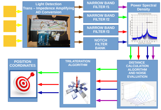
Fig. 2. Receiving system.
