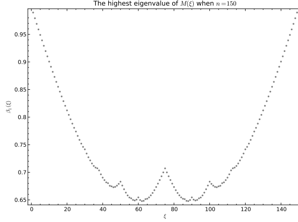
FIGURE 1. The top eigenvalues of M(\xi)
