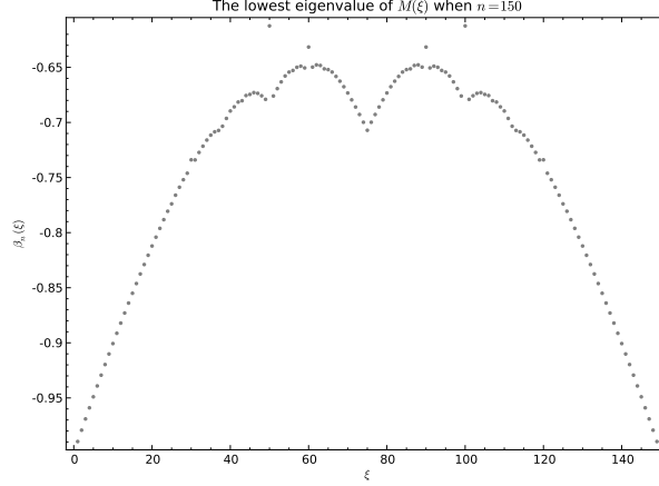
FIGURE 2. The lowest eigenvalues of M(\xi)
