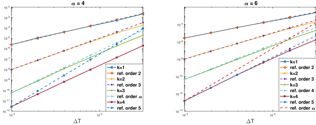
FIGURE 3. Orders of convergence of the error with respect to \Delta T , for \bar{\alpha} = 4 (left) and \bar{\alpha} = 6 (right), for different values of k \in \{1, 2, 3, 4\} , in the linear implicit Euler scheme case.
