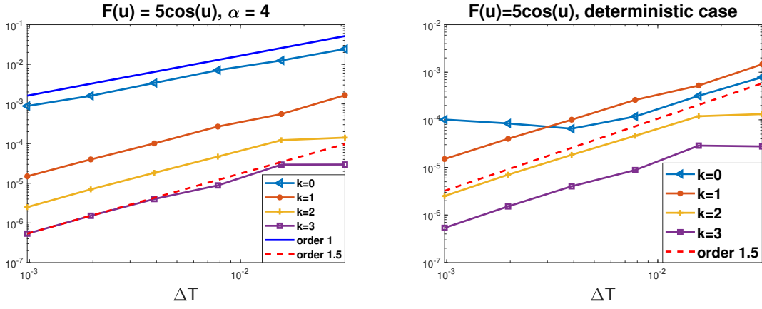
FIGURE 5. Orders of convergence of the error with respect to \Delta T , for additive noise case with \bar{\alpha} = 4 (left) and deterministic case (right), for nonlinear term F(u) = 5 \cos(u) and different values of k \in \{0, 1, 2, 3\} , in the linear implicit Euler scheme case.
