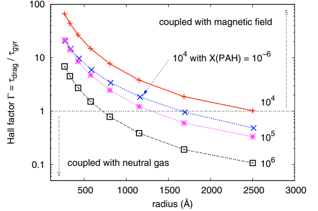
Fig. 3. The Hall factor, \Gamma = \tau_{\text{drag}}/\tau_{\text{gyr}} , as a function of the grain radius for a range of pre-shock densities, with T = 10\text{ K} and \zeta = 10^{-17}\text{ s}^{-1} , and with or without PAHs. The grains tend to be less coupled to the magnetic field at high density: the dependency \Gamma \propto n_H^{-1/2} is clear for environments with no PAHs. The presence of PAHs shifts the grain charge toward zero, thus reducing their Hall factor.
