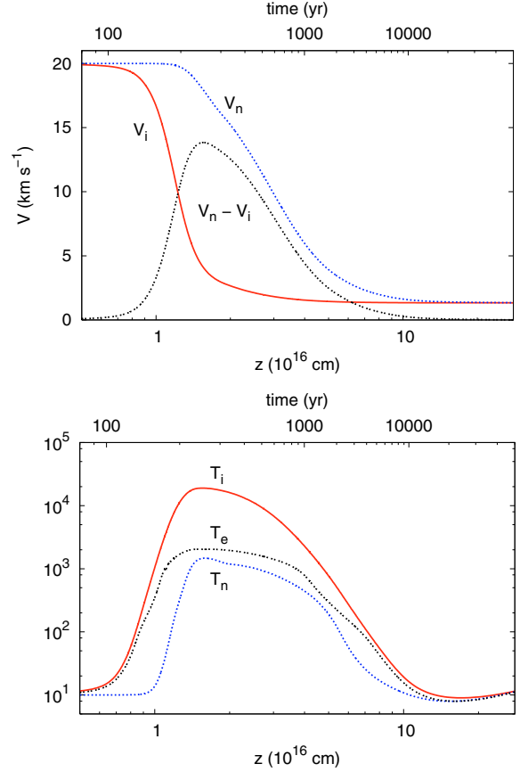
Fig. 4. Velocity and temperature profiles for a 20 km s -1 C shock propagating through our standard pre-shock conditions ( T = 10 K, n_{\text{H}} = 10^4 cm -3 , B = 100 μG and \zeta = 10^{-17} s -1 ). The shock ends approximately at 3 \times 10^4 yrs which corresponds to a shock length of \approx 0.06 pc. The upper axis indicates the neutral gas flow time t_n = \int dz/V_n .
