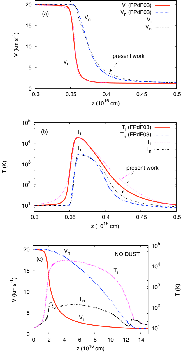
Fig. D.1. The velocity a ) and temperature b ) profiles for a C shock propagating in a cloud with proton density n_H = 10^6 \text{ cm}^{-3} , as obtained with the FPdF03 shock code assuming that the charged dust grains follow the ion motion, compared with the present work. c ) Velocity and temperature profiles for the same C shock but with no dust. At such high density, dust grains fully dominate the coupling in momentum between magnetic field and neutral gas. Neglecting dust, the shock length is increased by more than an order of magnitude.
