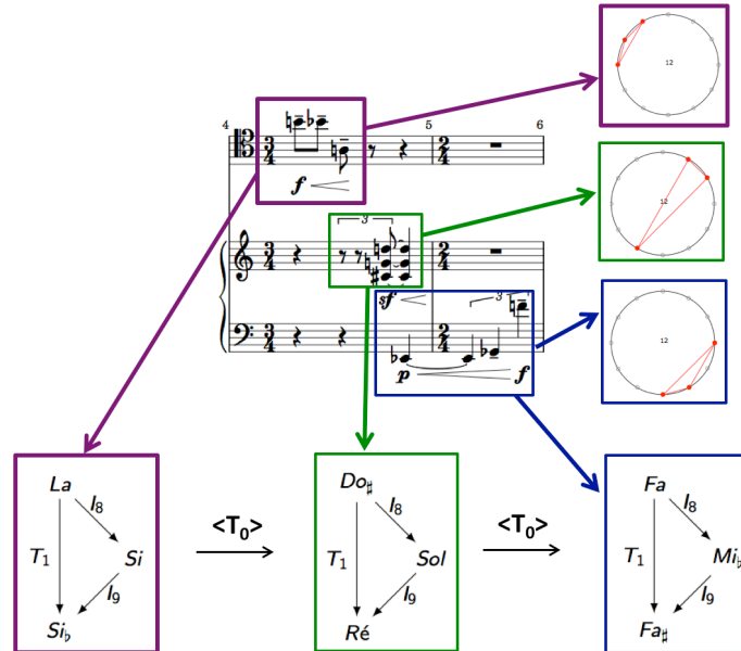
Figure 5. Three chords belonging to Anton Webern's Drei Kleine Stücke , Op. 11/2 which literally share the same type of transpositions and inversions without being in the same orbit under the action of the cyclic, dihedral or affine groups. See [36].
