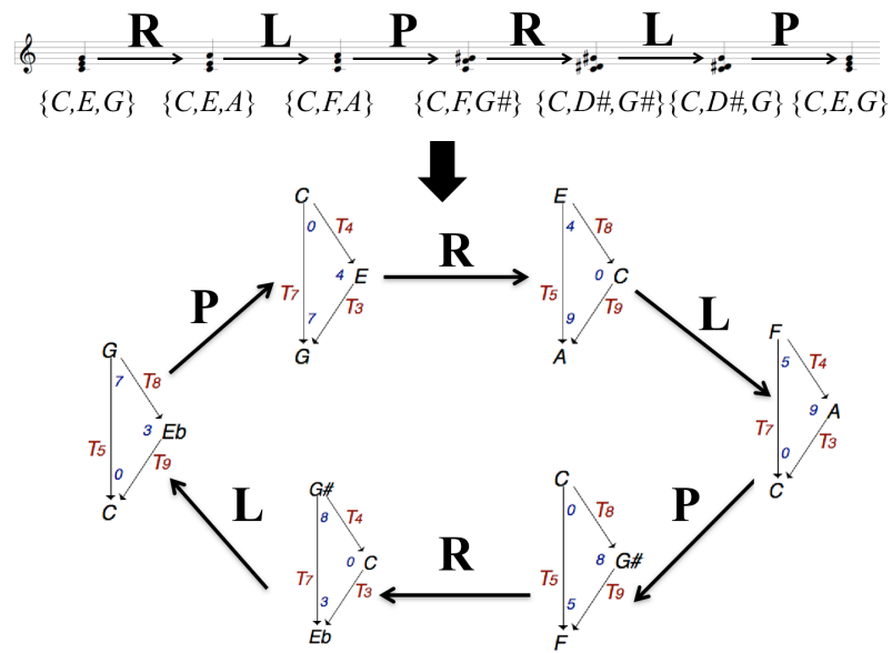
Figure 4. The hexagonal cycle generating the Tonnetz and represented in a categorical framework displaying the transformations between major and minor chords viewed as labelled graphs with vertices corresponding to the notes and arrows corresponding to transposition operations. See [36].
