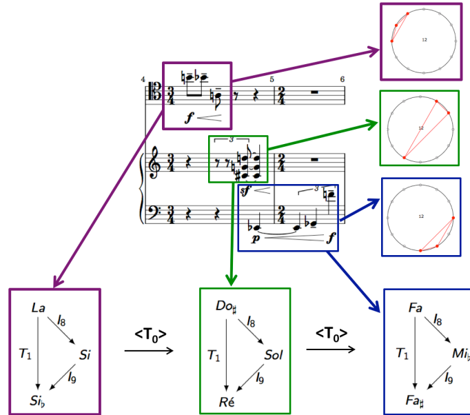
Figure 5. Three chords belonging to Anton Webern's Drei Kleine Stücke , Op. 11/2 which literally share the same type of transpositions and inversions without being in the same orbit under the action of the cyclic, dihedral or affine groups. See [36].
