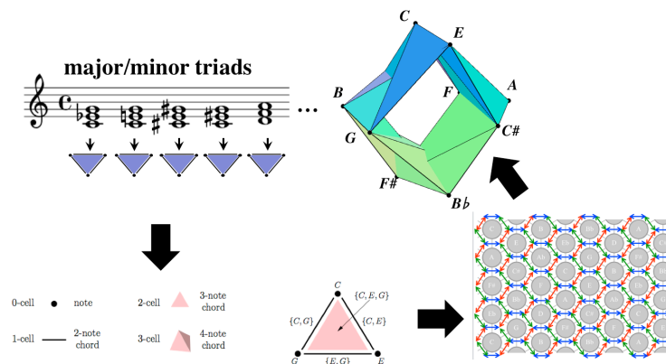
Figure 3. The Tonnetz as a simplicial complex obtained by self-assembly of major and minor chords viewed as 2-cells. See [14].
