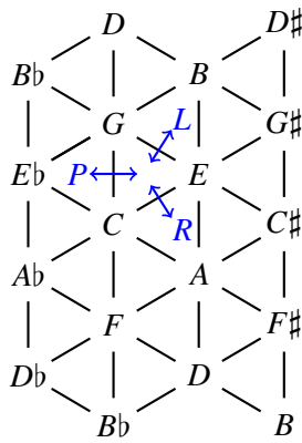
Figure 1: The neo-Riemannian Tonnetz and the P , L and R operations
