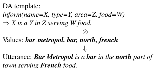
Figure 1: Dialog act example.
