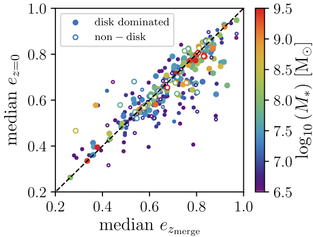
Figure 10. Median eccentricities at merger time e_{\text{zmerge}} against median eccentricity at z = 0 e_{z=0} for satellites accreted onto Milky Way mass haloes in EAGLE. The points are coloured by the stellar mass of the accreted galaxies at the time of the merger, M_* . As in Fig. 9, point sizes denote the number of stellar particles in the satellite, and the open points show satellites accreted onto galaxies with no clear disc component. Debris which falls below the dashed unity line has been circularized following accretion, whereas the debris above this line has been radialized after accretion. The majority of debris has a similar e at z = 0 to the time at which it was accreted, but a few accreted satellites are circularized/radialized following accretion. High mass satellite debris has undergone the least change in median e .
