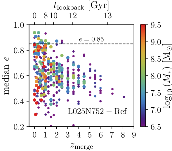
Figure B2. The merger time z_{\text{merge}} of satellites accreted onto Milky Way mass haloes in the L025N752-Ref simulation against the median eccentricity e of their stellar debris at z = 0 , produced via an equivalent analysis to that which produced Fig. 9. The upper envelope of z = 0 eccentricity for a given merger time is reproduced in this lower resolution simulation, albeit with a different calibration of the subgrid model, demonstrating the ‘weak’ convergence of this result.
