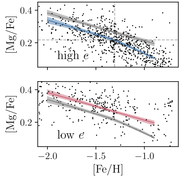
Figure 6. Best-fit models for [\text{Mg}/\text{Fe}] as a function of [\text{Fe}/\text{H}] for the high- and low- e k -means groups (shown top and bottom, respectively). The best-fit model is shown by the blue and red lines, with the 95 per cent confidence interval marked by the banded blue and red regions either side of this line (the fit for the other group is shown in each panel for reference). The raw data are shown by the black scatter points. The high- e group is well-fit by a model with a break at [\text{Fe}/\text{H}] = -1.31^{+0.03}_{-0.06} and [\text{Mg}/\text{Fe}] = 0.22^{+0.01}_{-0.08} , as indicated by the dashed crosshair. The low- e group is better fit by a single linear relation in the same range of [\text{Fe}/\text{H}] . The position of the models also demonstrates the slightly higher [\text{Mg}/\text{Fe}] of the low- e group.
