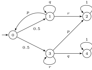
Fig. 1: pMC \mathcal{M}_1
