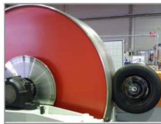
Figure 1. Typical drum testing machine/external surface test [12].
