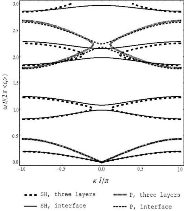
Fig. 3. Comparison between the band gaps for a one-dimensional phononic crystal made of three layers and the band gaps calculated for two layers separated by an interface. In the two situations, \varepsilon is 1.0 \times 10^{-3}l . The large dashed lines and the tiny dotted lines represent the dispersion curves of SH and P waves, respectively, for the crystal made of three layers. The solid lines and the small dashed lines represent the dispersion curves of SH and P waves, respectively, for the crystal made of two layers separated by the interface.
