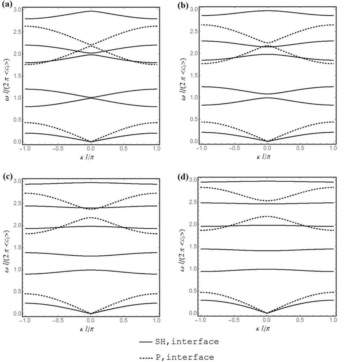
Fig. 4. Case I. Band gaps for a one-dimensional phononic crystal with imperfect interfaces of increasing interface thickness: a) \epsilon/l = 0 ; b) \epsilon/l = 1.0 \times 10^{-3} ; c) \epsilon/l = 5.0 \times 10^{-3} ; d) \epsilon/l = 1.0 \times 10^{-2} . The solid lines and the dashed lines represent the dispersion curves of SH and P waves, respectively.
