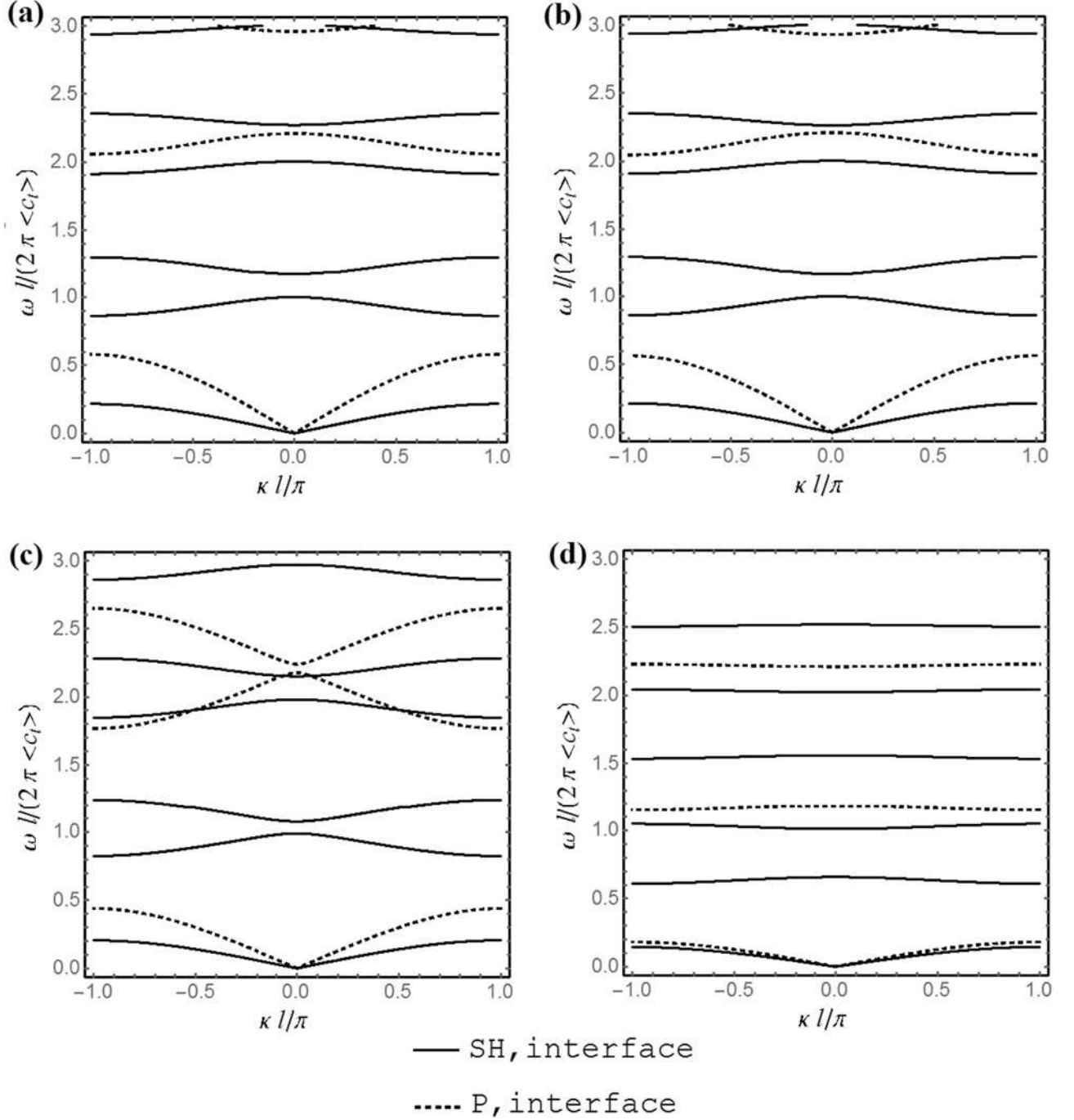
Fig. 6. Case III. Band gaps for a one-dimensional phononic crystal with imperfect interfaces of increasing interface density: a) \zeta / \langle \rho \rangle = 1.0 \times 10^{-2} ; b) \zeta / \langle \rho \rangle = 1.0 \times 10^{-1} ; c) \zeta / \langle \rho \rangle = 1.0 ; d) \zeta / \langle \rho \rangle = 1.0 \times 10^1 . The solid lines and the dashed lines represent the dispersion curves of SH and P waves, respectively.
