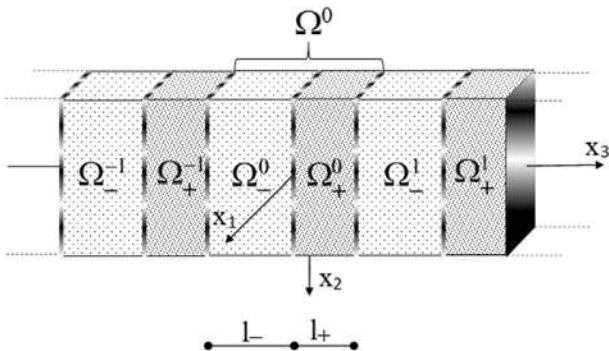
Fig. 2. Sketch of a 1D phononic crystal as a layered periodic structure obtained by alternating different layers separated by higher order imperfect interfaces.
