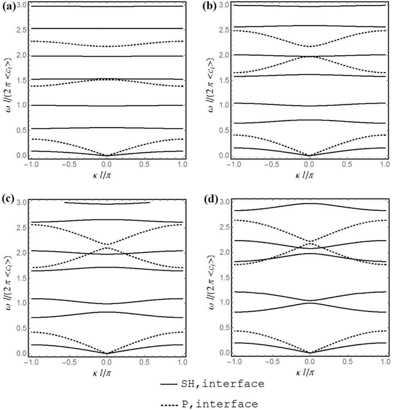
Fig. 5. Case II. Band gaps for a one-dimensional phononic crystal with imperfect interfaces of increasing interface stiffness: a) \lambda / \langle \lambda \rangle, \mu / \langle \mu \rangle = 1.0 \times 10^{-2} ; b) \lambda / \langle \lambda \rangle, \mu / \langle \mu \rangle = 5.0 \times 10^{-2} ; c) \lambda / \langle \lambda \rangle, \mu / \langle \mu \rangle = 1.0 \times 10^{-1} ; d) \lambda / \langle \lambda \rangle, \mu / \langle \mu \rangle = 5.0 \times 10^{-1} . The solid lines and the dashed lines represent the dispersion curves of SH and P waves, respectively.
