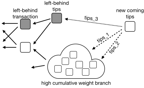
Fig. 5. Tips selection with left-behind tips protection
