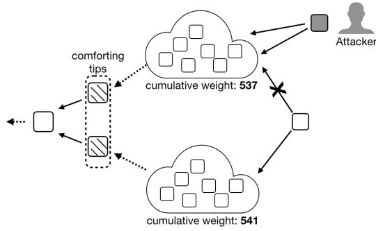
Fig. 2. Illustration of a splitting attack scenario.
