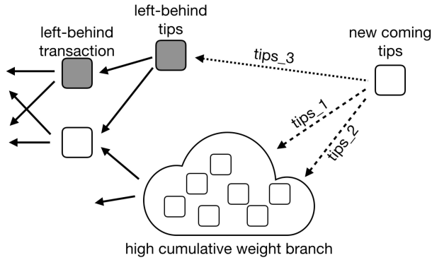
Fig. 5. Tips selection with left-behind tips protection
