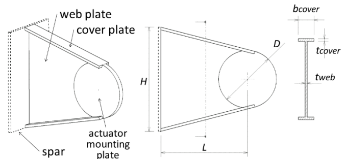
Figure 8. Attachment geometry
