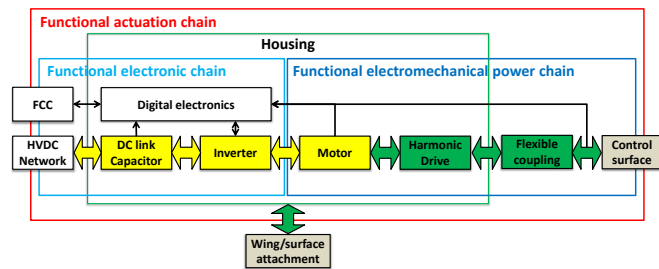
Figure 1. Rotary EMA architecture
