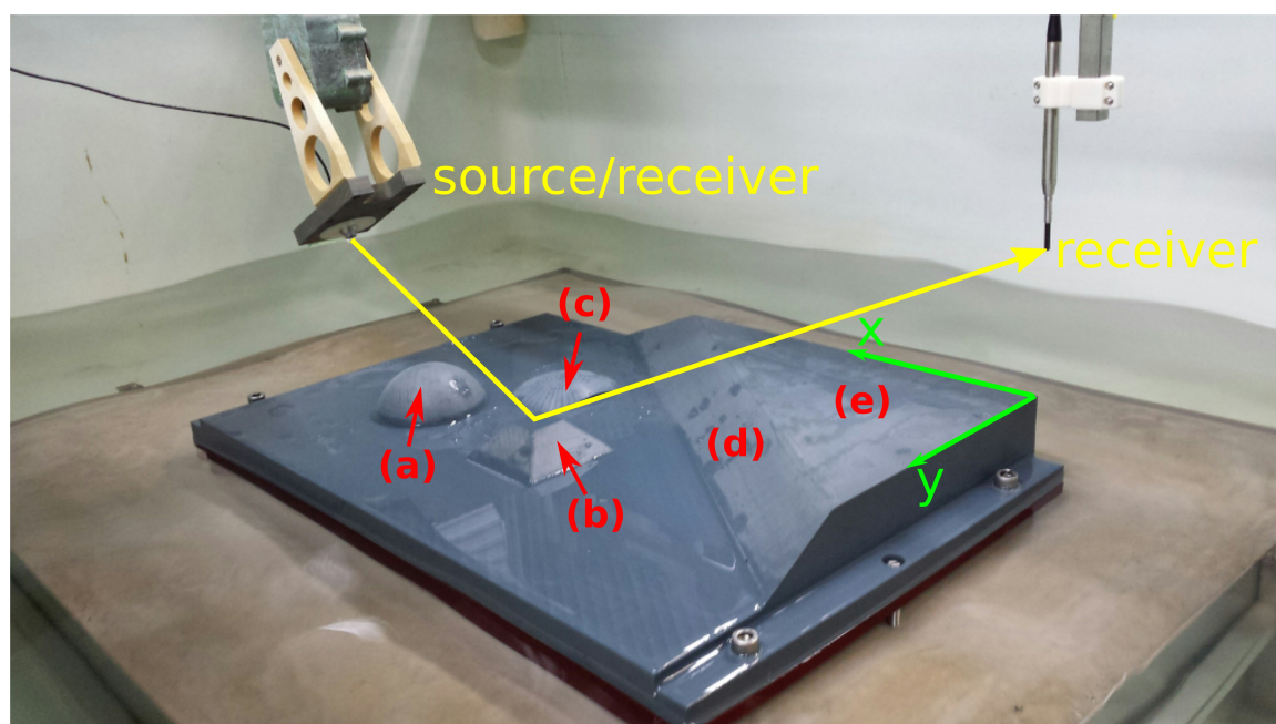
18 19 20 21 22 23 24 25 26 27 28 29 30 31 32 33 34 35 36 37 38 39 Figure 1. Illustration of the small-scale seismic experiments performed in the water tank. 40 41 The Marseille-Benchic model contains a dome (a), a truncated pyramid (b), a truncated 42 dome (c), a ramp (d) and an elevated plateau (e). The model is illuminated by a 43 piezoelectric transducer (on the left). In offset configuration, the wavefield is recorded by 44 a hydrophone (on the right). 45 46 47 48 49 50 51
