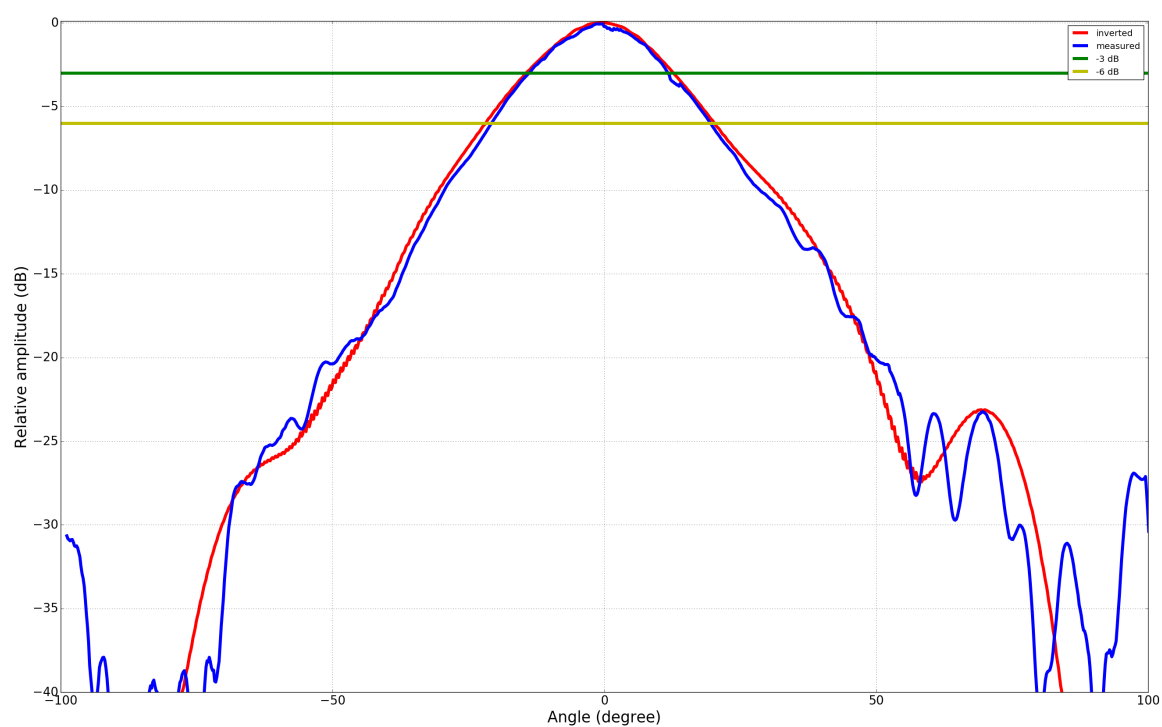
20 21 22 23 24 25 26 27 28 29 30 31 32 33 34 35 36 37 38 39 40 41 42 43 Figure 9. Comparison of the measured (blue) and inverted (red) radiation patterns of the 44 45 transducer in offset configuration. The amplitude is maximal opposite to the transducer 46 47 ( 0^\circ ). 48 49 50 51 52 53 54 55 56 57 58 59 60
