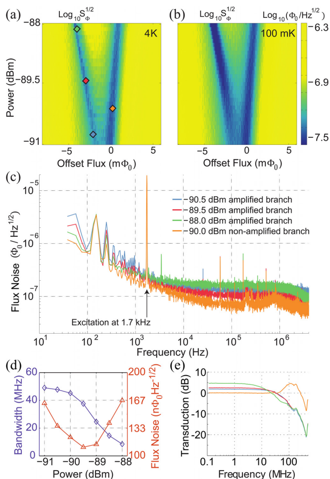
FIG. 3. (a) and (b) Estimated flux noise based on the data from Fig. 2 and the noise model described in the text for T=4 K, and T=100 mK. (c) Measured flux noise at 4 K and at different bias points on flux noise estimation. In order to simultaneously measure the transduction coefficient, an ac signal with an amplitude of 20 \mu\Phi_0 and frequency of 1.7 kHz was applied to one of the field coils and the voltage noise was obtained by averaging the noise floor between 50 kHz and 100 kHz. (d) Dependence of the bandwidth and flux noise on excitation power on the parametrically amplified branch. (e) Corresponding transduction of excitation vs. frequency for the different bias points shown in (a) and (c).
