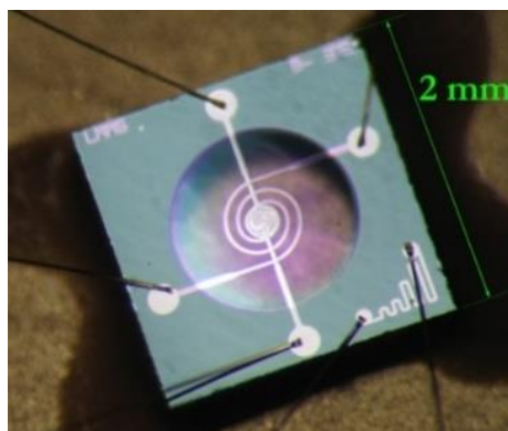
Fig. 1 Image of the gas sensor silicon platform (LAAS).
