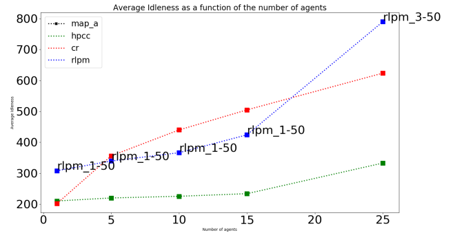
Fig. 5: Normalised average idleness of the evaluated strategy for the map A in ordinate for the three maps and the population sizes of agents in abscissa.
