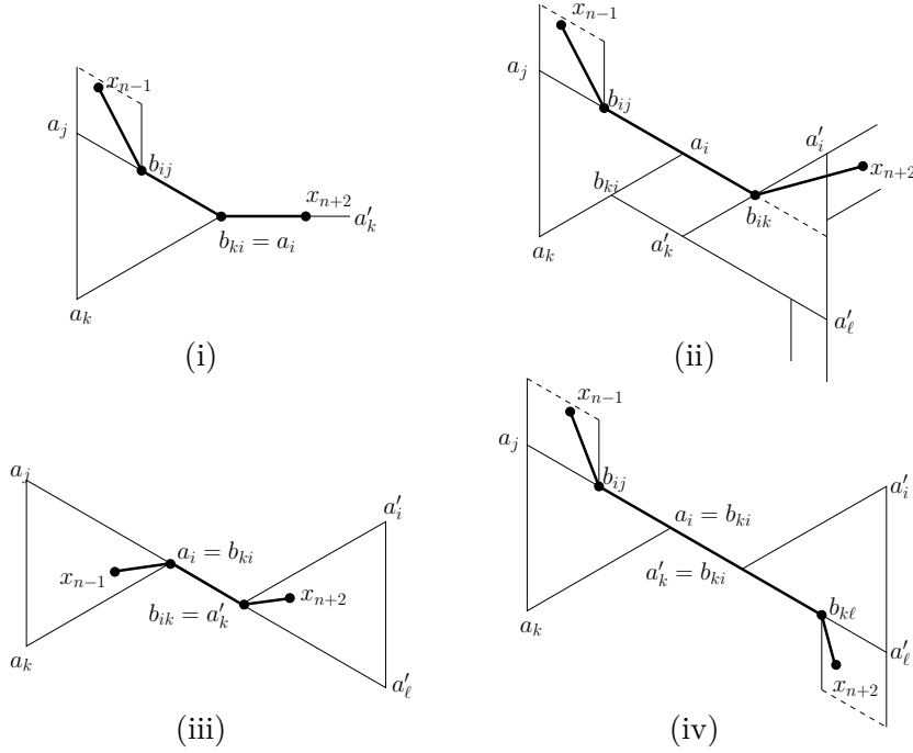
FIGURE 14. Singular segment in a geodesic in \widetilde{K} : the four cases.
