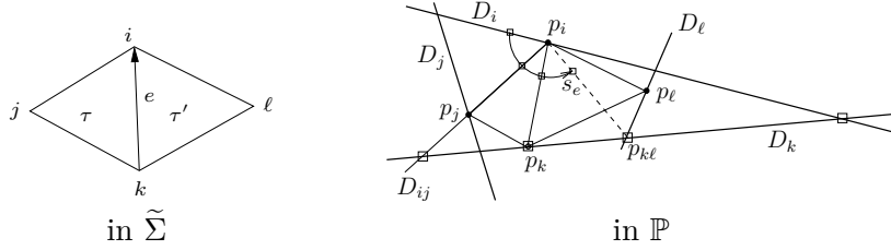
FIGURE 10. The edge invariant s_e associated with an edge e .
